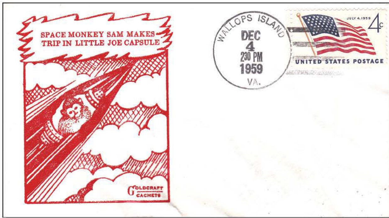
Capsule aerodynamics (LJ-6) and abort at max Q (LJ-1A) is followed by launch of "Sam". The name Sam comes from the acronym School of Aerospace Medicine.
